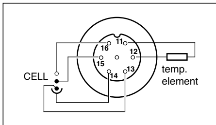
Fig. 25 SC42/SC49 4-electrode connector (top view)
