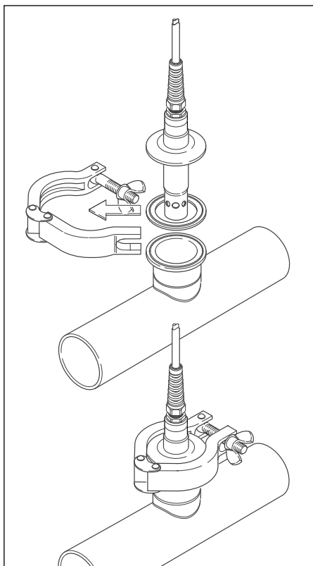
Fig. 6 Mounted SC4A-E-SB (SC) sensor with tri-clamp
